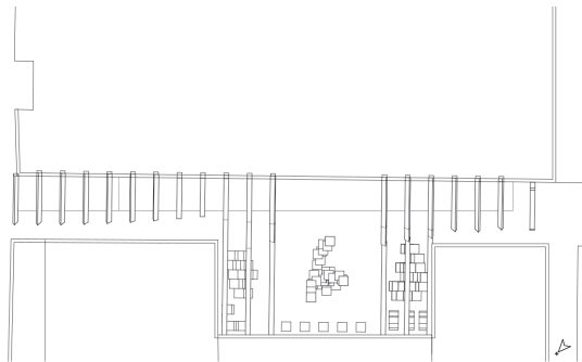
Roof Plan and Elevation
